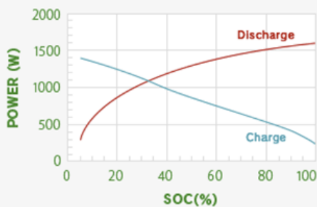
UN test results Example of charge-discharge characteristics (25°C, BOL)
