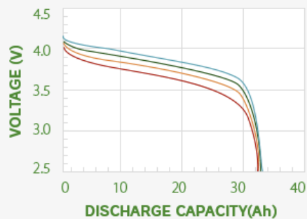
Cell performance Example of discharge profiles (25°C, BOL)
