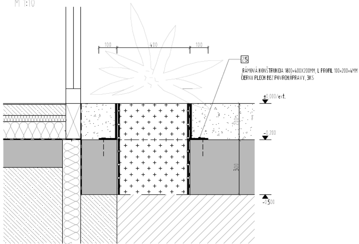
REZ M 1:10
