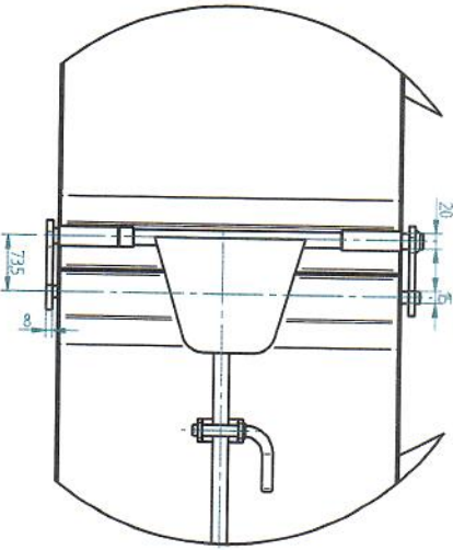
DETAIL C 15
