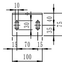
LEFT VIEW
