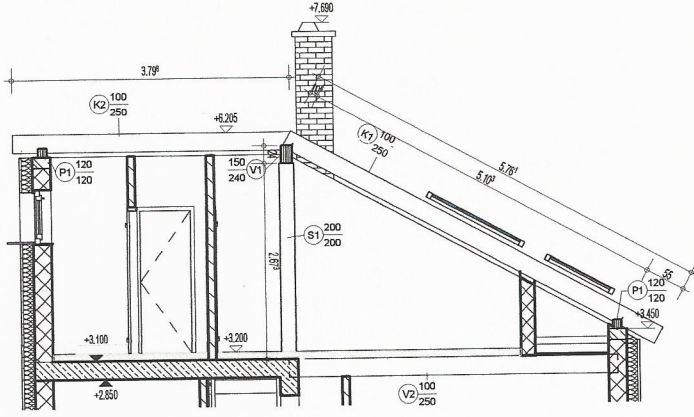
Rez Krov 1
