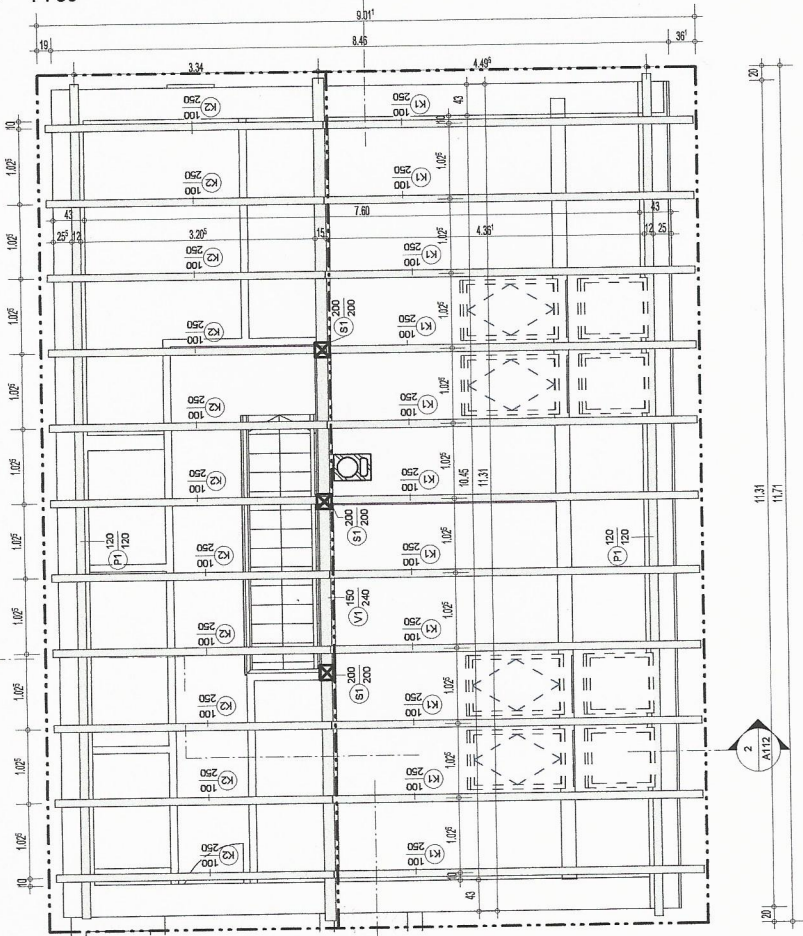
Rez Krov 1
