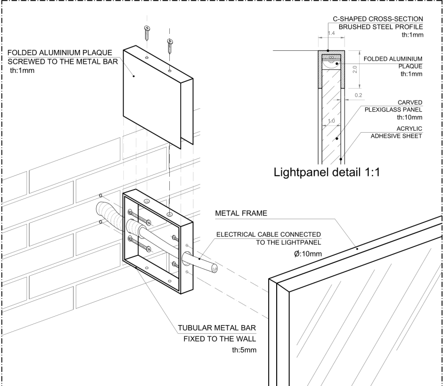
Light panel detail 1:1
