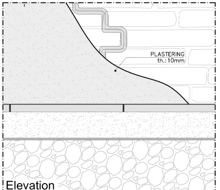
Section, elevation
