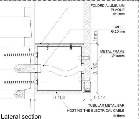
Wall mounting devices
