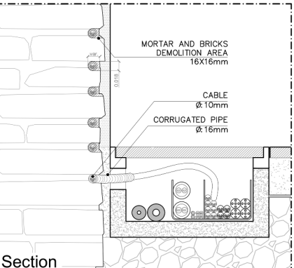
Electrical supply for light panels
