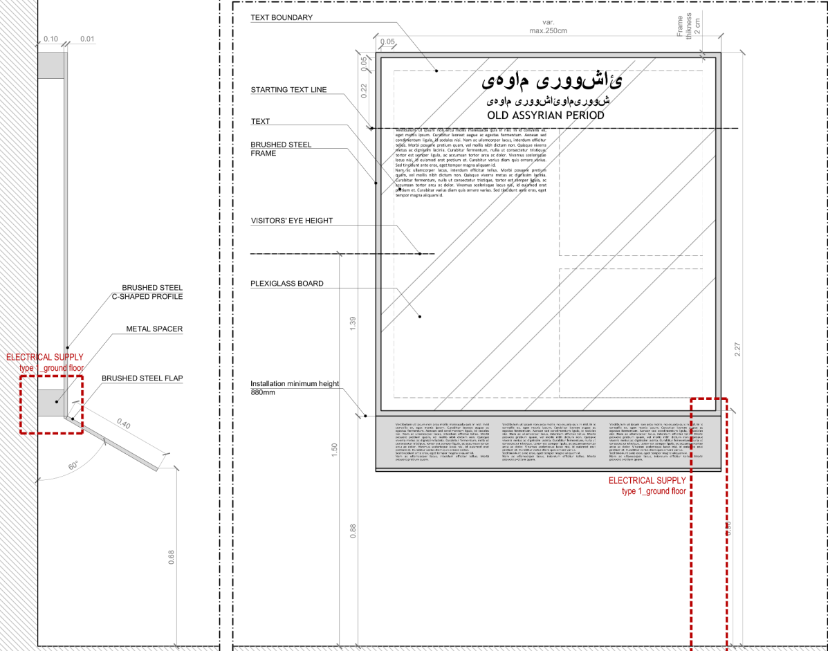
Standard lightpanel with lower flap
