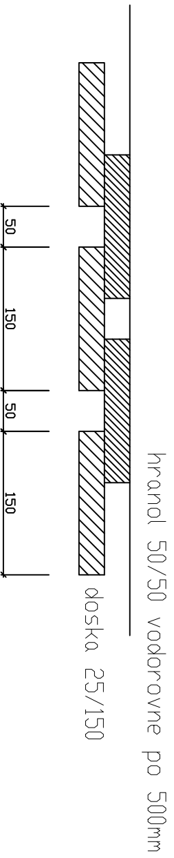
DETAIL A
