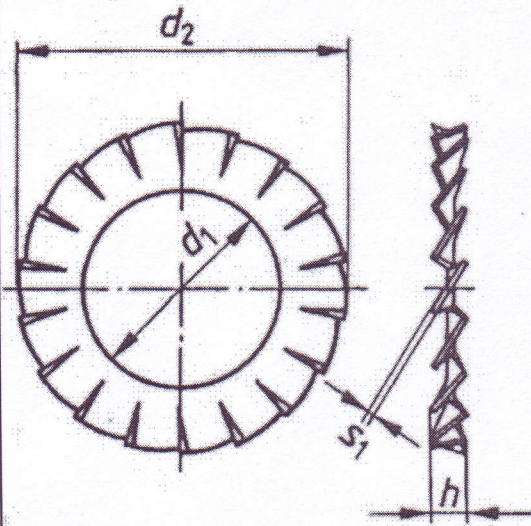
Type A, with external teeth
