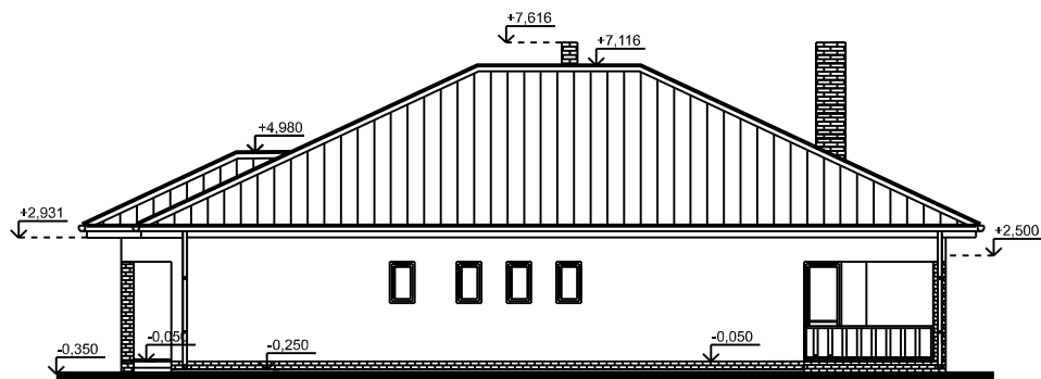
POHLAD SEVERNÝ
