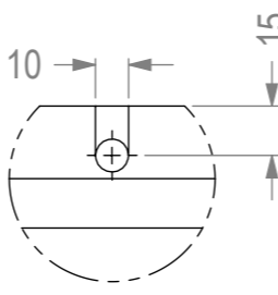
VIEW B SCALE 1 : 2.5
