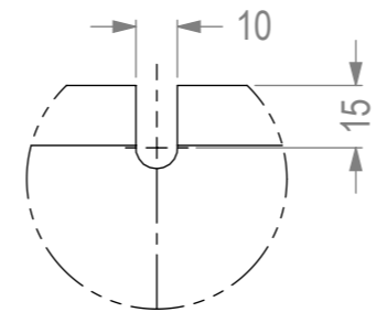
VIEW B SCALE 1 : 2
