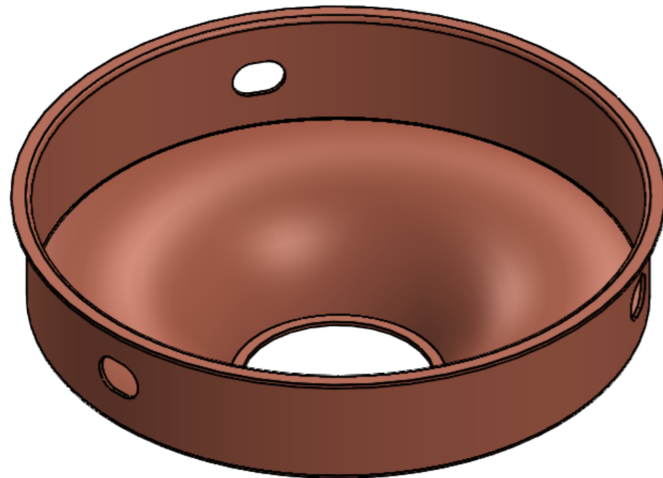
Polished copper Part no.: 2083LP01A Polished 1060 Aluminium Surface treatment: Anodized Color: Copper
