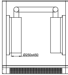
RIGHT SIDE VIEW MUFFLER DETAY
