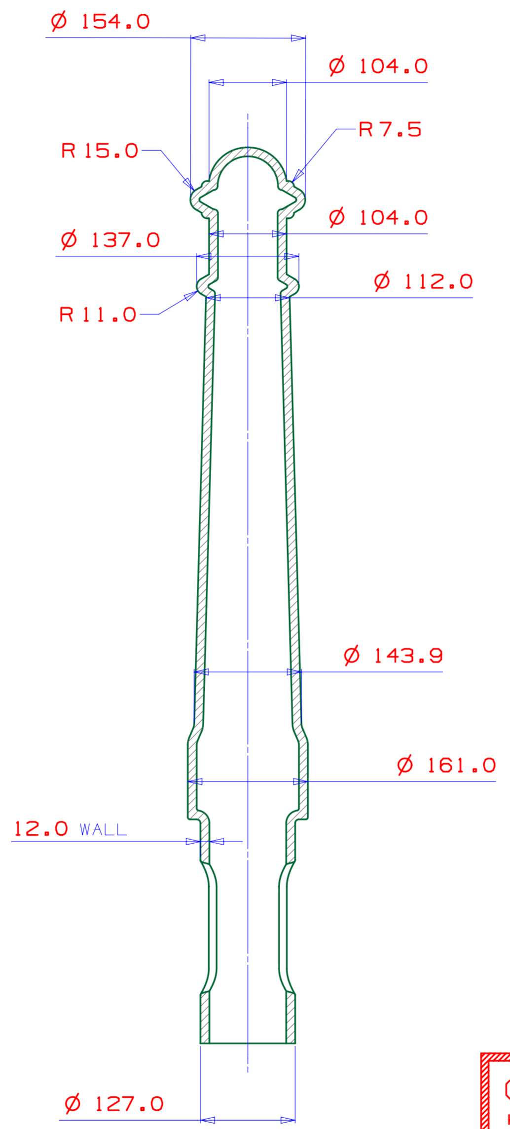
SECTION A - A
