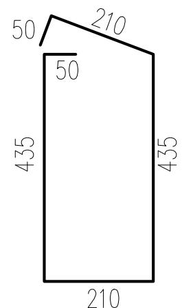
∅ R 6 – 1,39 m 16 ks
