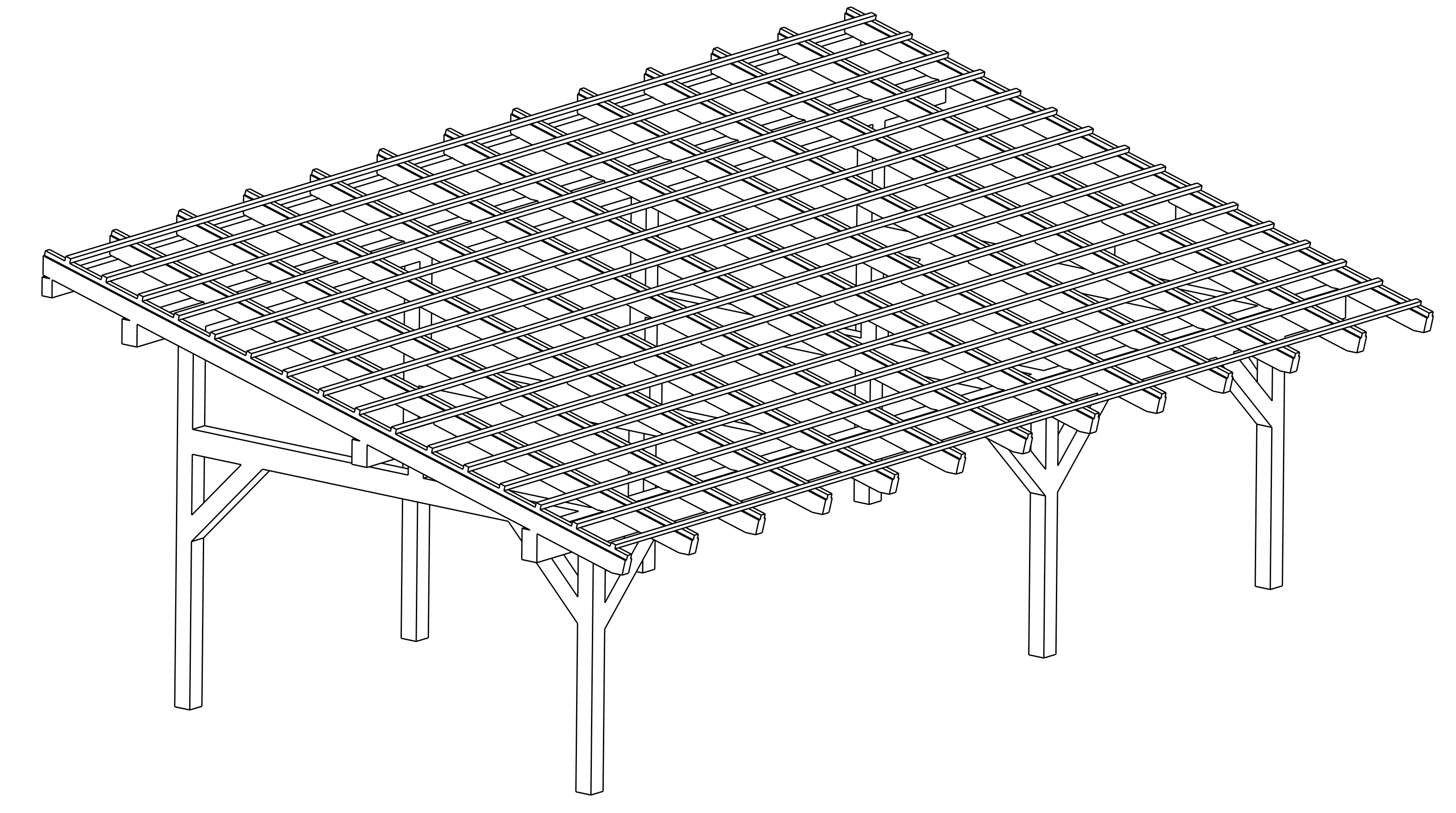
Isometric view Scale: 1:25
