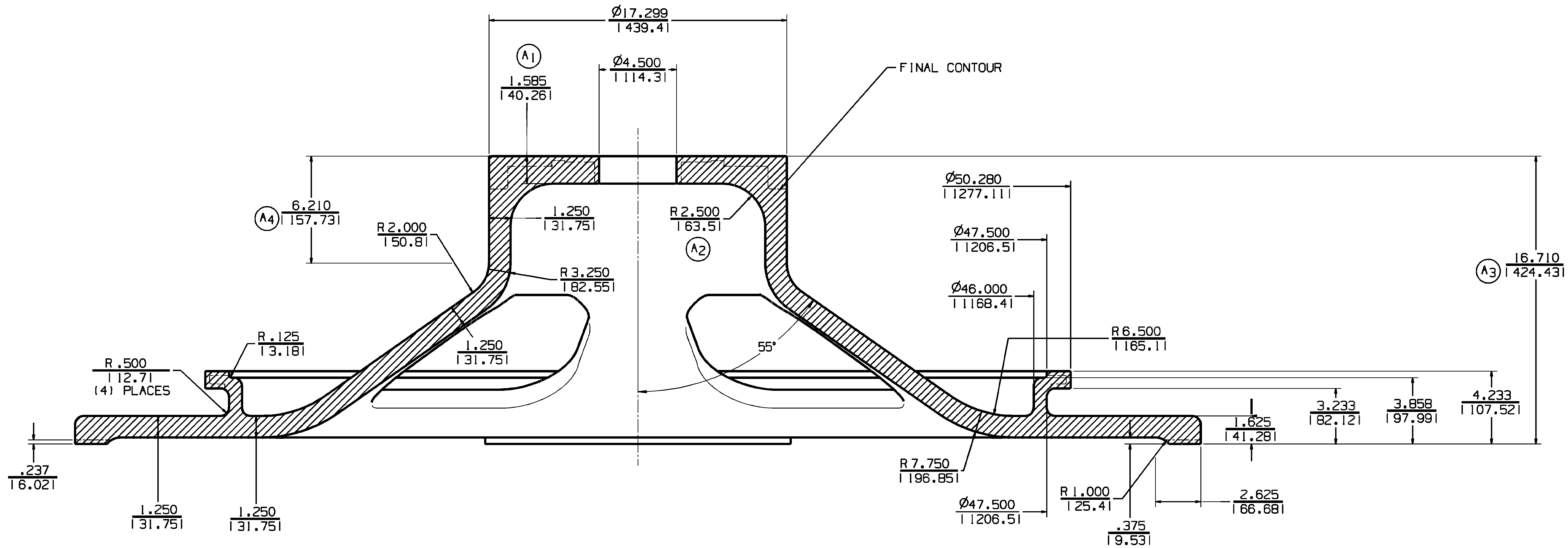
SECTION B-B
