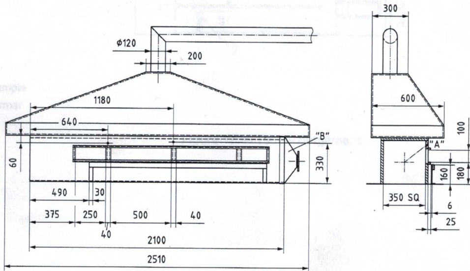
Figure 15 — Exhaust Hood
