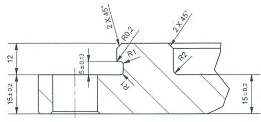
B (1:1)
